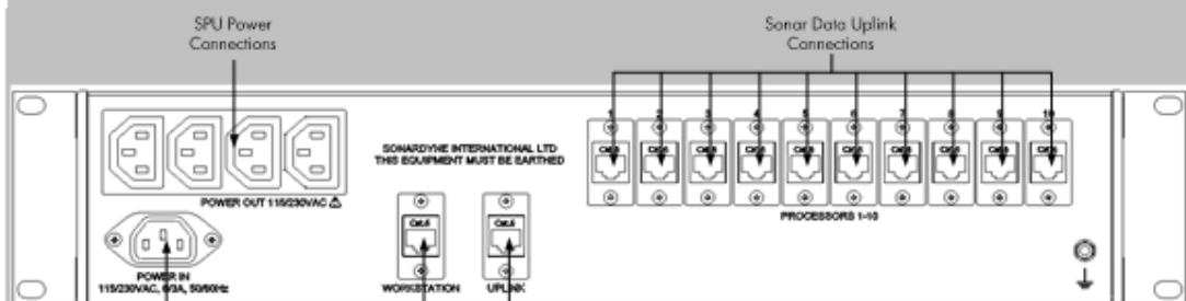
Input Power Connection
