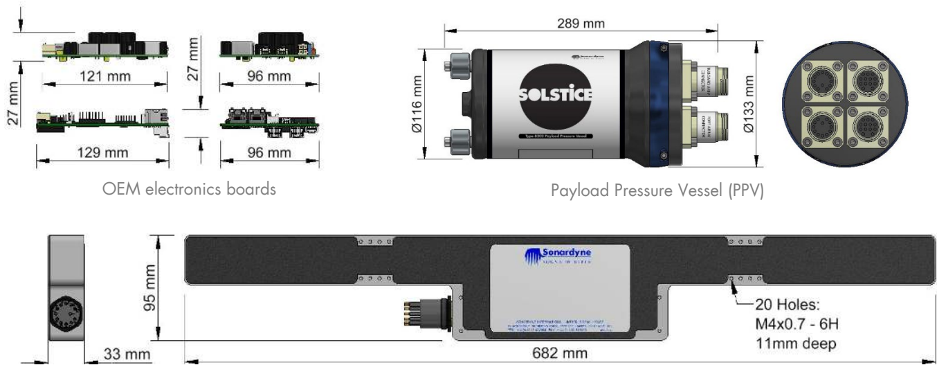
Solstice Array shown. Electronics can be supplied as OEM or in a Payload Pressure Vessel (PPV) both shown.
